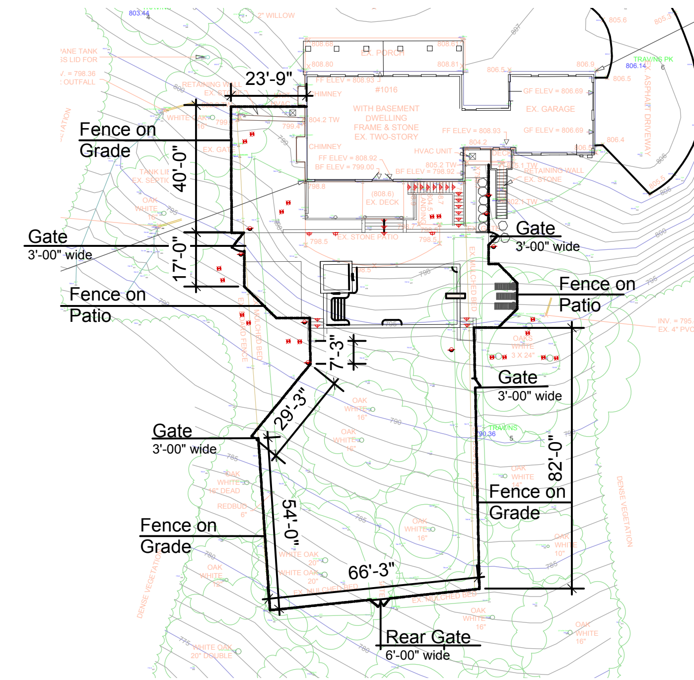
Fence Layout Plan scale 1" = 30'-00"
